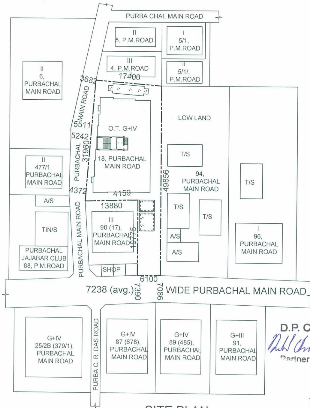
SITE PLAN SCALE:- 1:600
